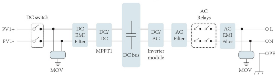
Circuit block diagram
